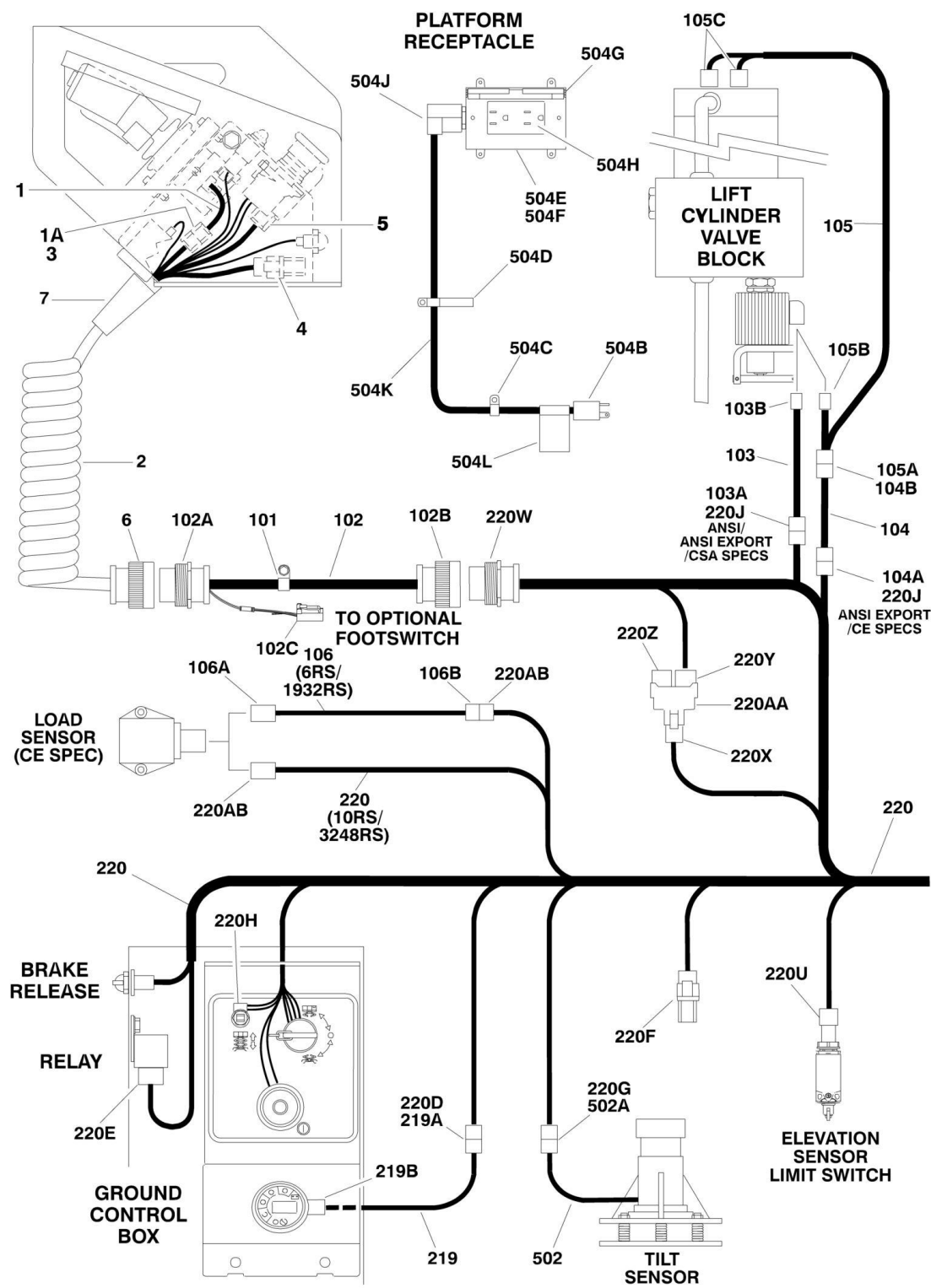
FIGURE 7-1. ELECTRICAL COMPONENTS INSTALLATION
