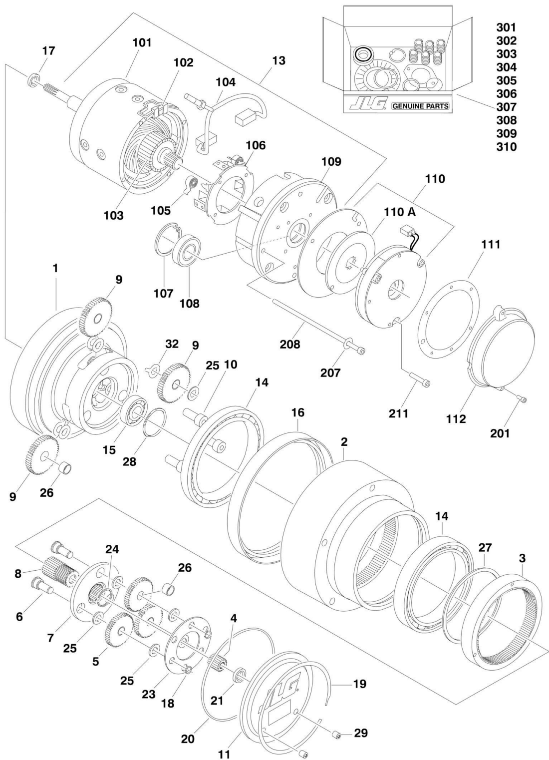
FIGURE 1-5. WHEEL DRIVE ASSEMBLY
